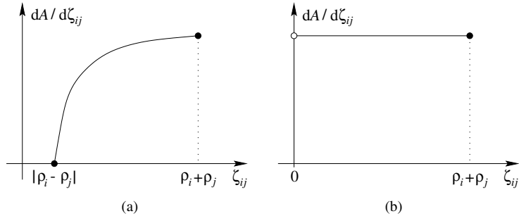
Fig. 4. (a) The graph for \varrho_i \neq \varrho_j , in which case the area derivative is positive at \zeta_{ij} = \varrho_i + \varrho_j and zero at \zeta_{ij} = |\varrho_i - \varrho_j| . (b) The graph for \varrho_i = \varrho_j , in which case the area derivative is a positive constant over the entire interval, except for \zeta_{ij} = 0 , where it is undefined.
